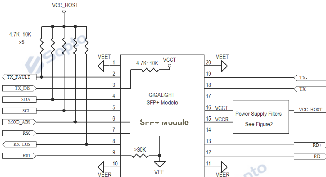
Host-Module Interface
