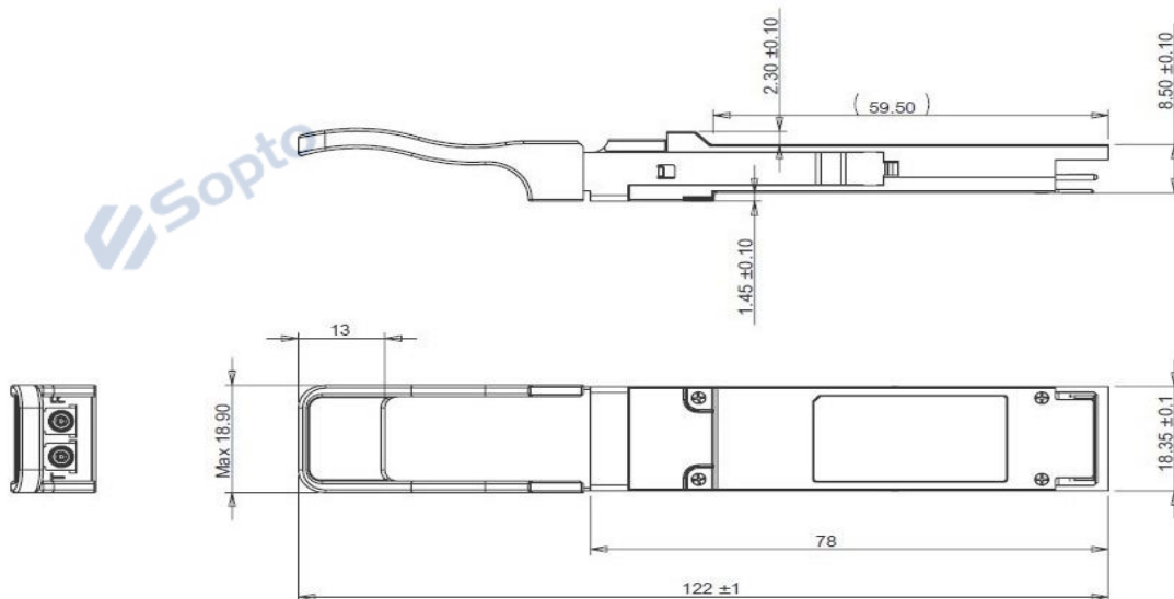
Figure 4. Mechanical Outline
