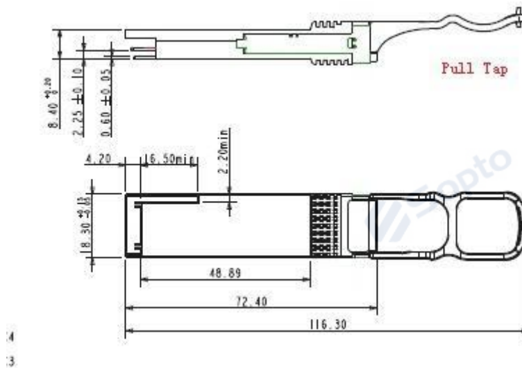
Figure9. Mechanical Specifications
