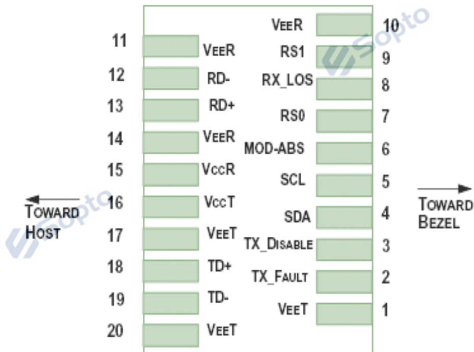
Figure1.Elecctrical Pin-out Details
