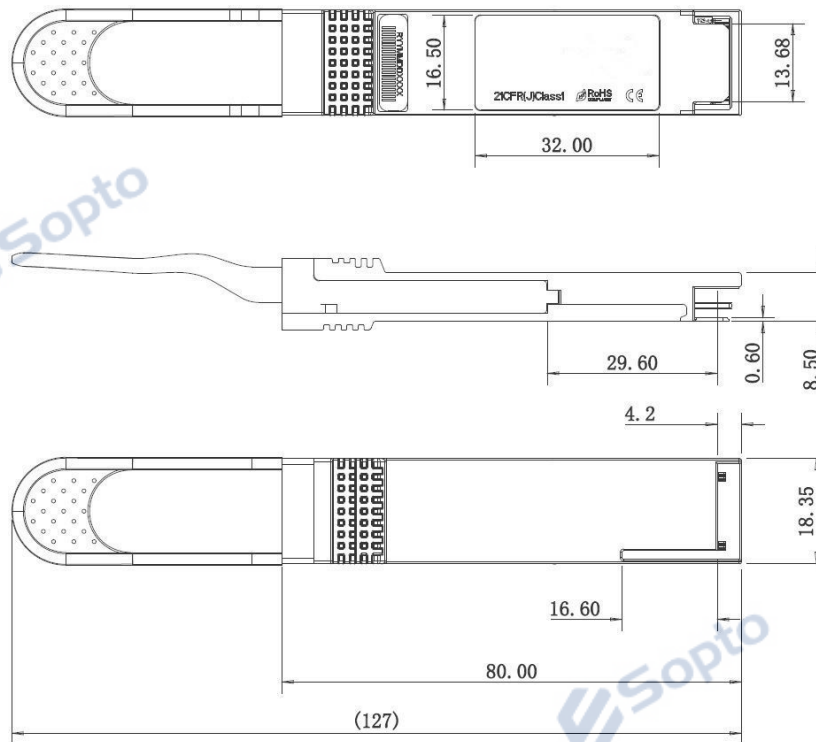
Figure10. Mechanical Specifications
