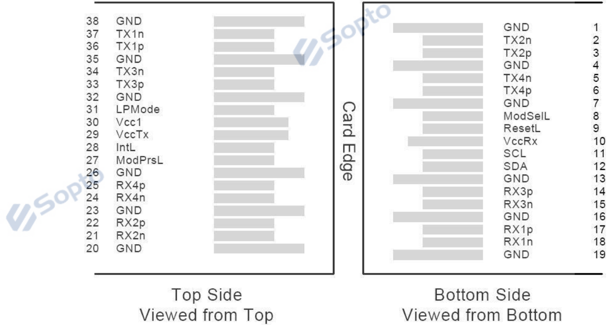
Figure 2. Electrical Pin-out Details
