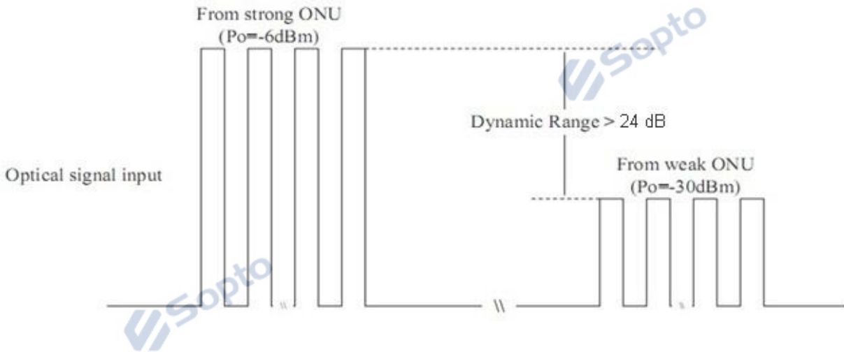
Figure2 Burst_mode Receiver Dynamic range in EPON system
