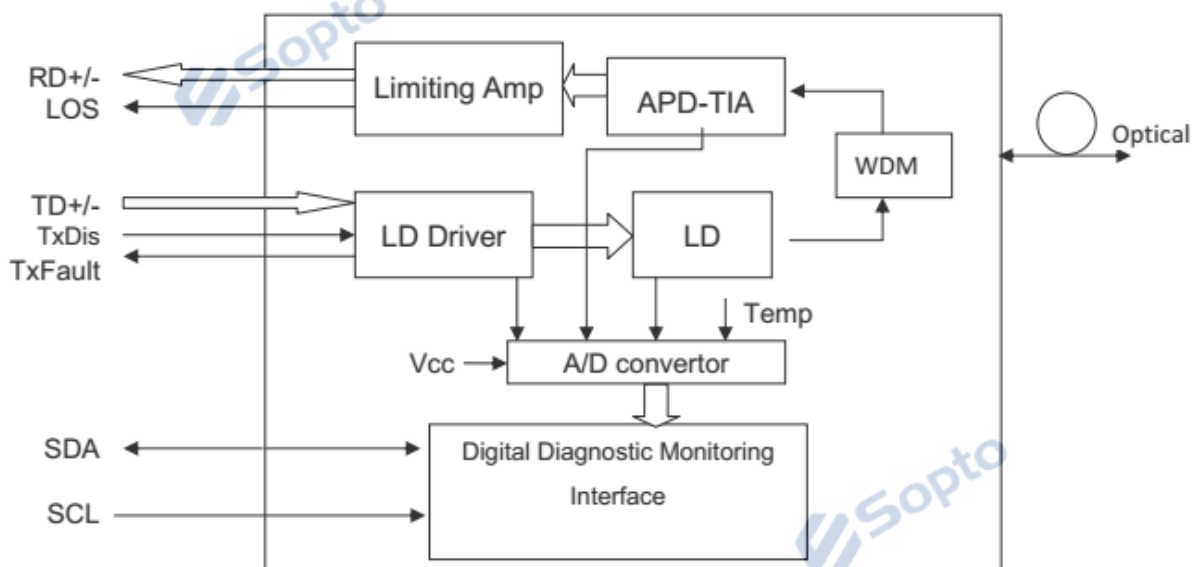
Fig 1 Transceiver Block Diagram
