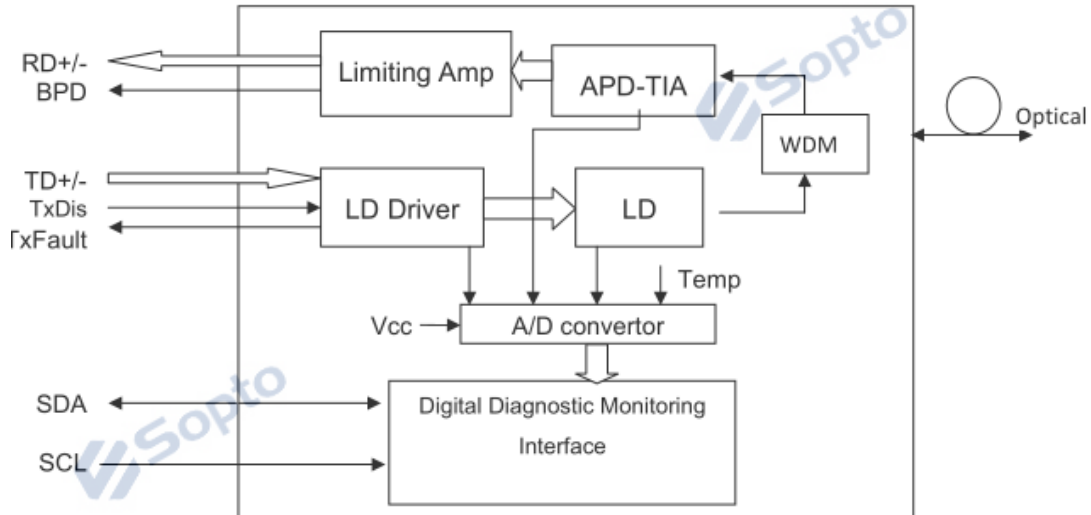
Fig 1 Transceiver Block Diagram
