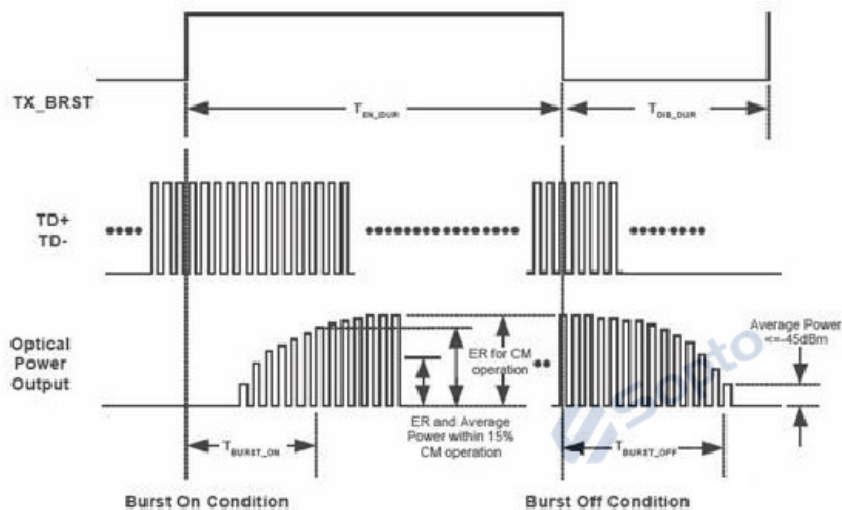
Tx Burst control: Logic '1' Tx ON
