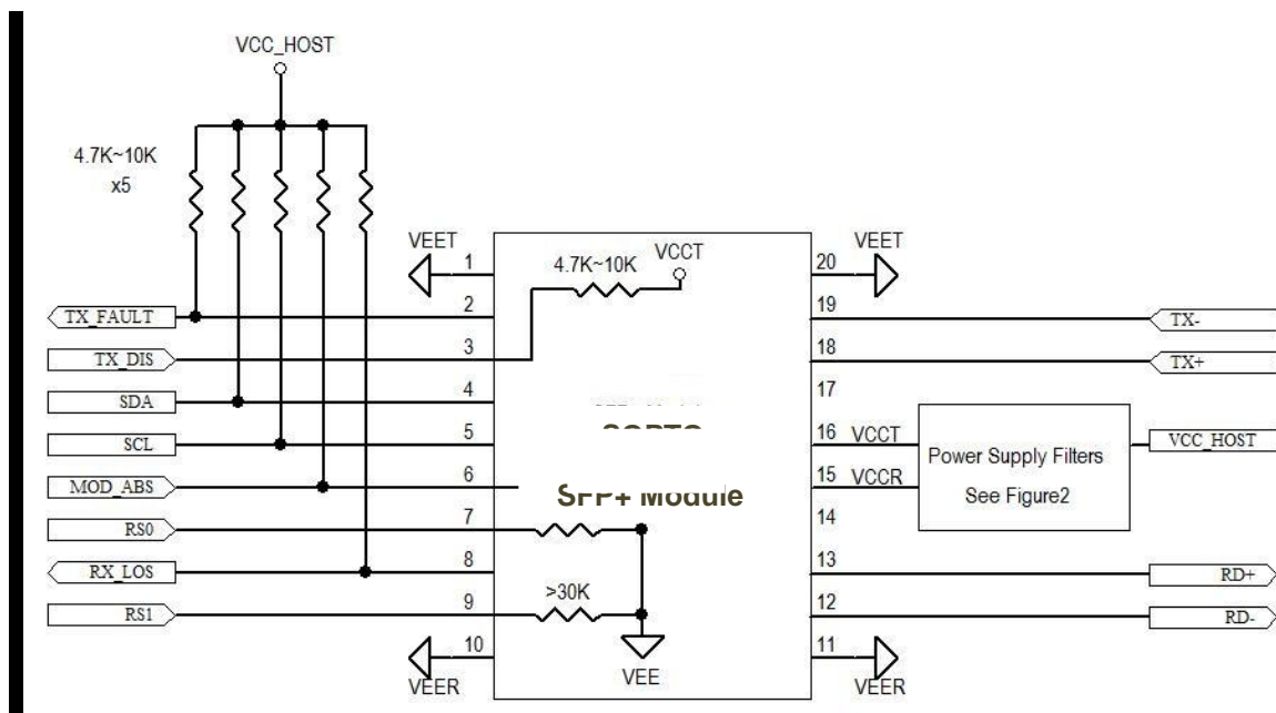
Figure4. Host-Module Interface
